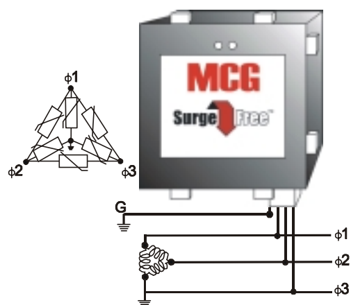
3 Phase, 3W+GND
